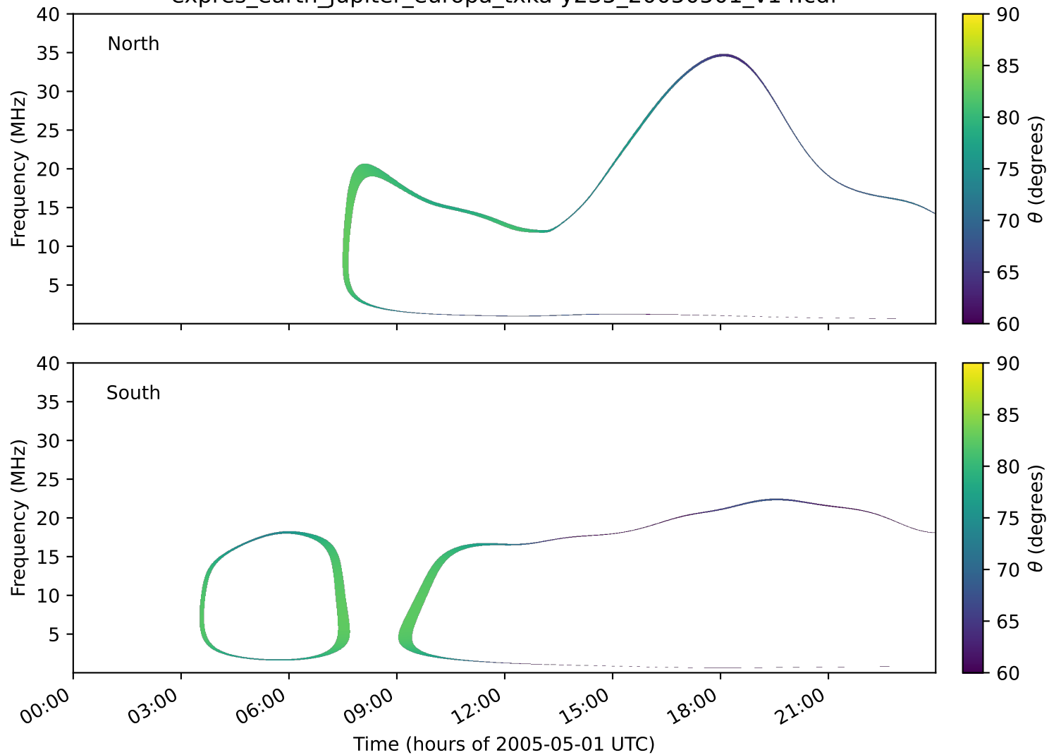
expres_earth_jupiter_europa_txka-y235_20050501_v14.cdf
