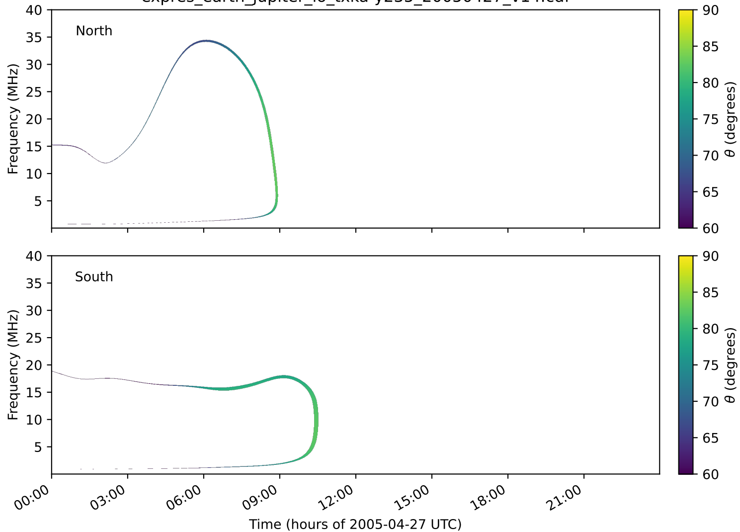
expres_earth_jupiter_io_txka-y235_20050427_v14.cdf
