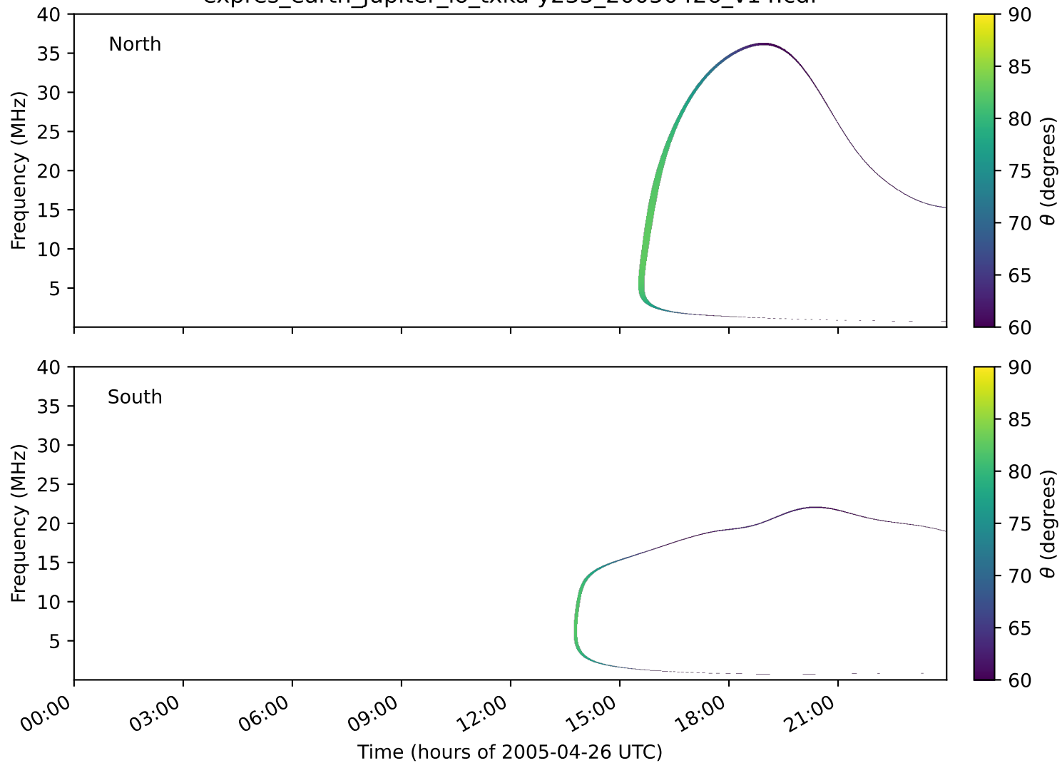
expres_earth_jupiter_io_txka-y235_20050426_v14.cdf
