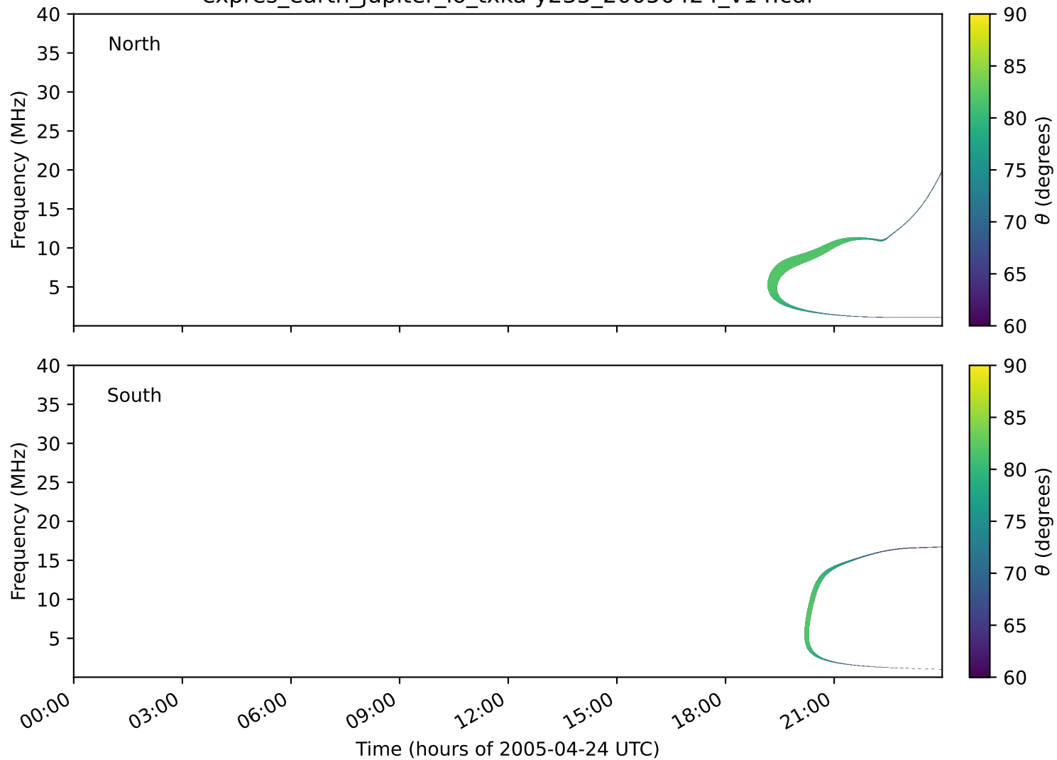
expres_earth_jupiter_io_txka-y235_20050424_v14.cdf
