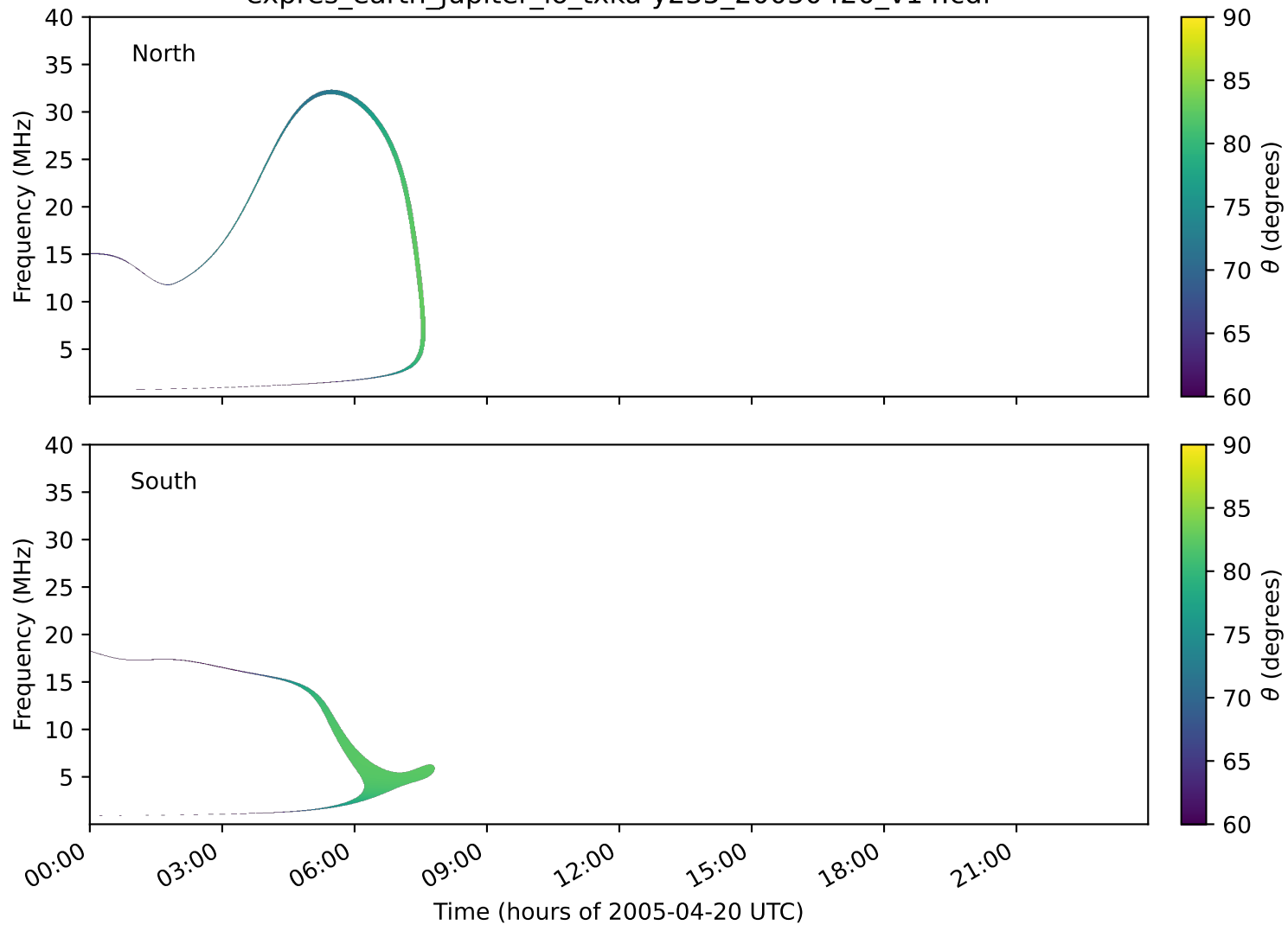
expres_earth_jupiter_io_txka-y235_20050420_v14.cdf
