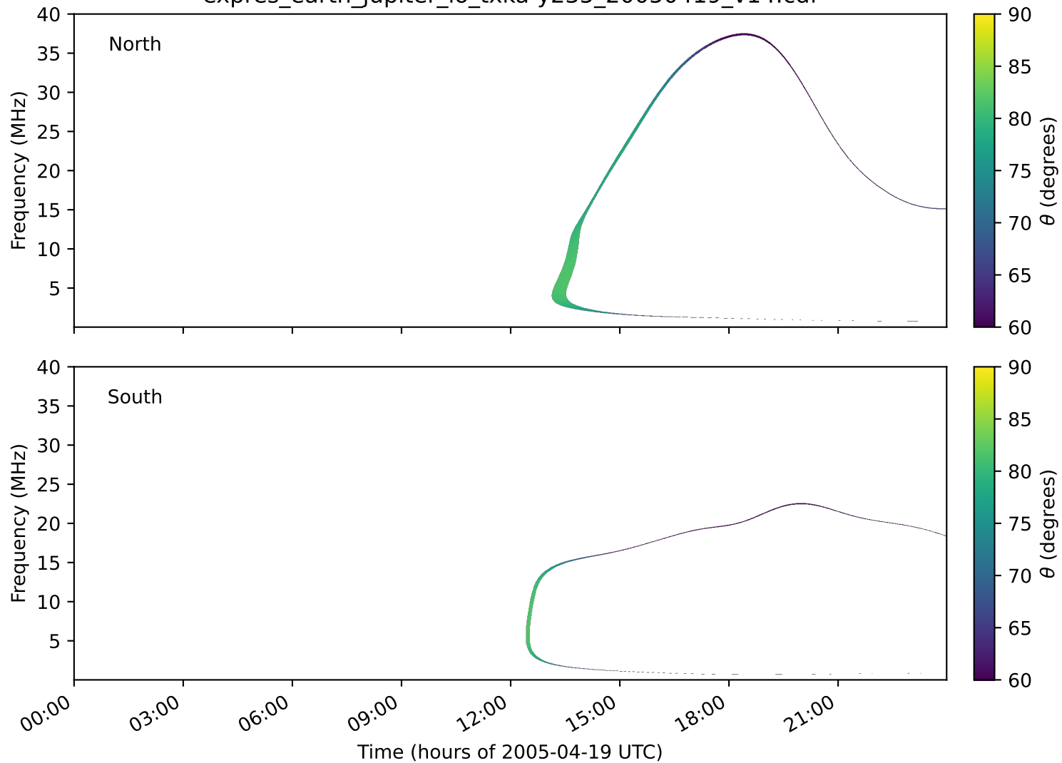
expres_earth_jupiter_io_txka-y235_20050419_v14.cdf
