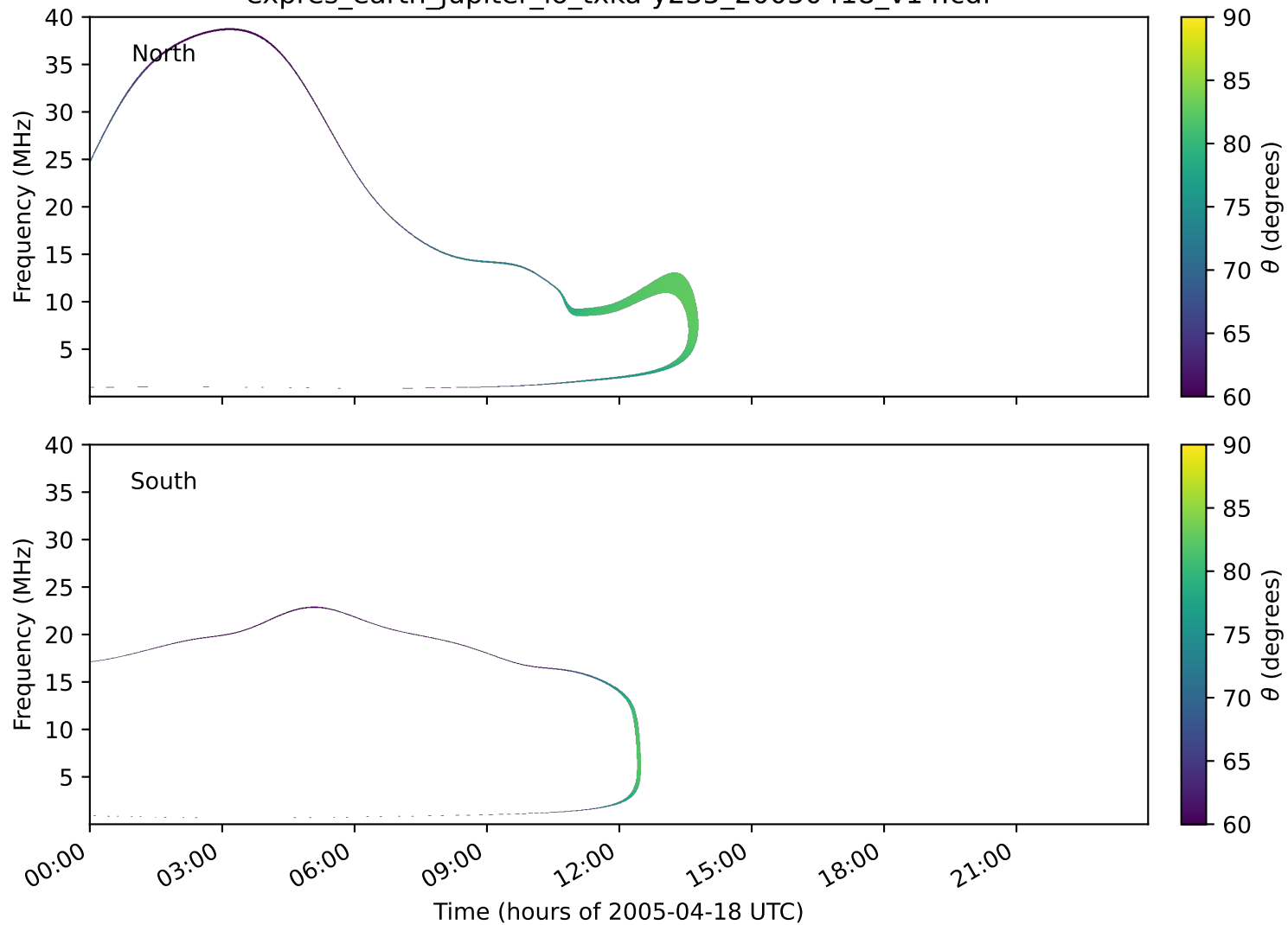
expres_earth_jupiter_io_txka-y235_20050418_v14.cdf
