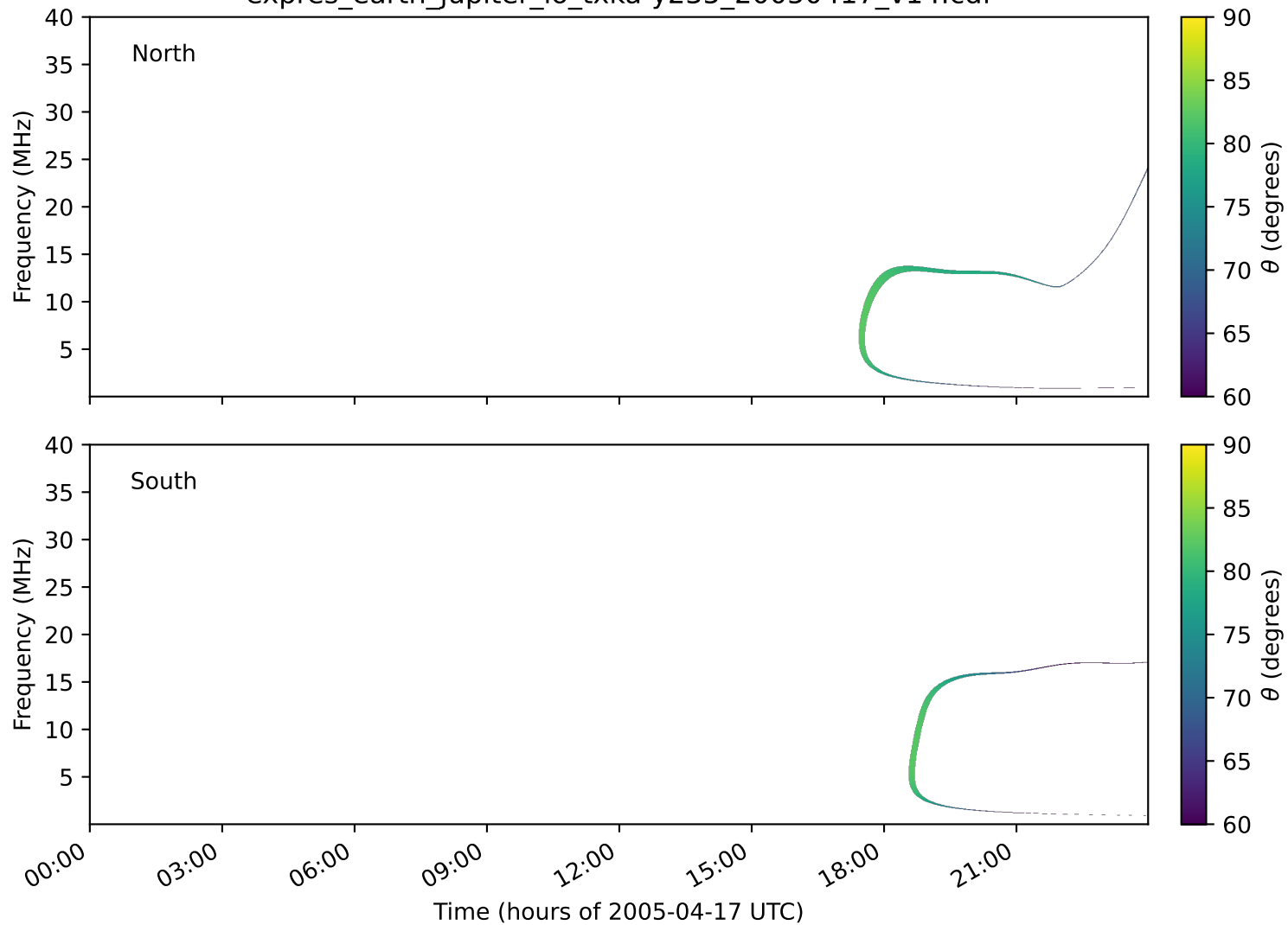
expres_earth_jupiter_io_txka-y235_20050417_v14.cdf
