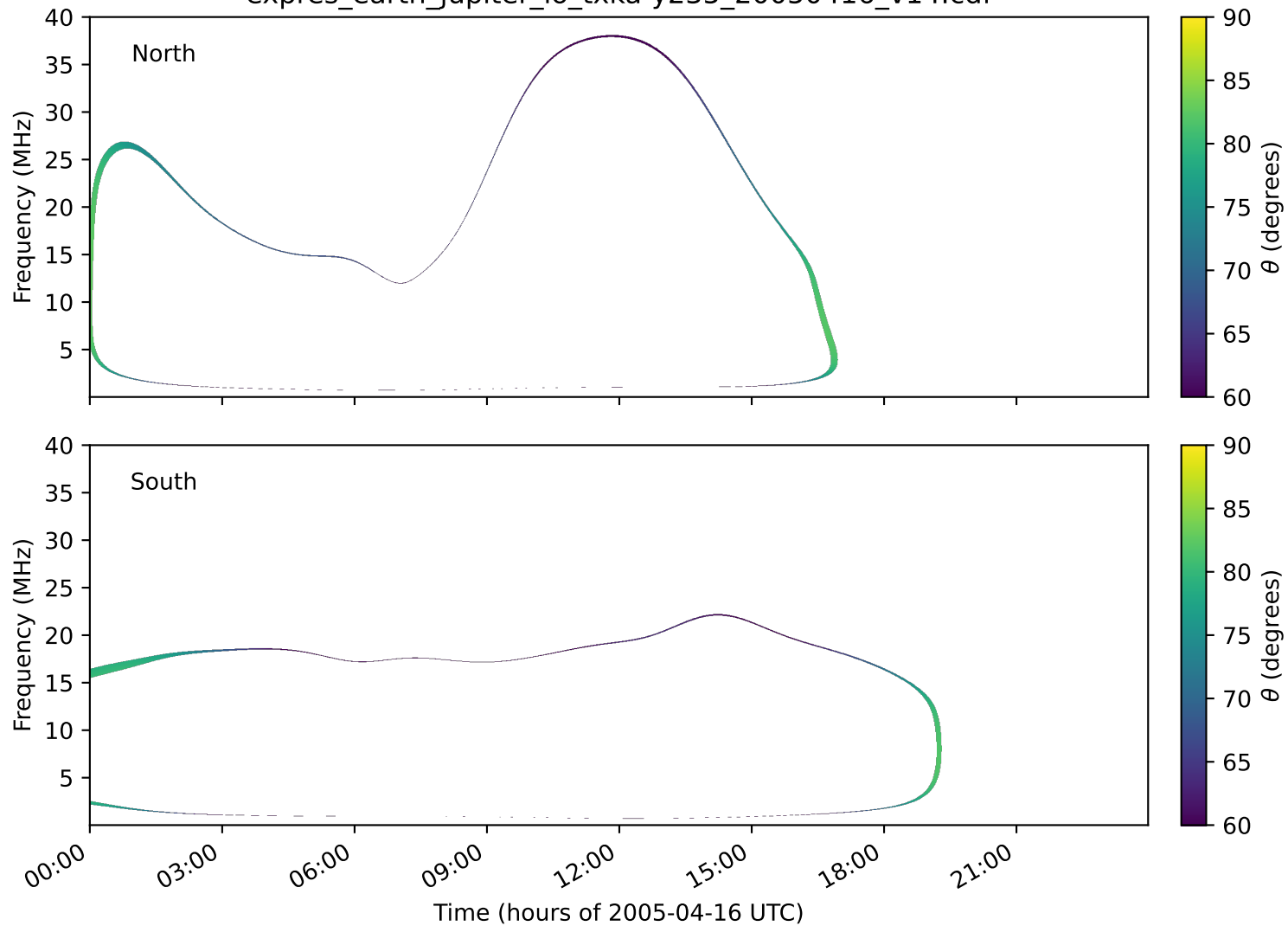
expres_earth_jupiter_io_txka-y235_20050416_v14.cdf
