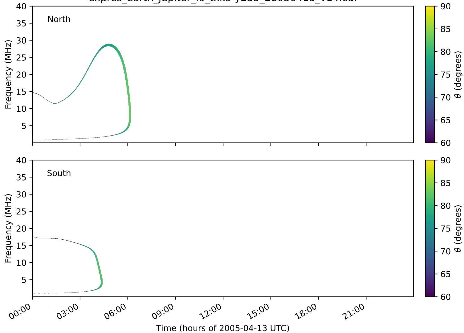
expres_earth_jupiter_io_txka-y235_20050413_v14.cdf
