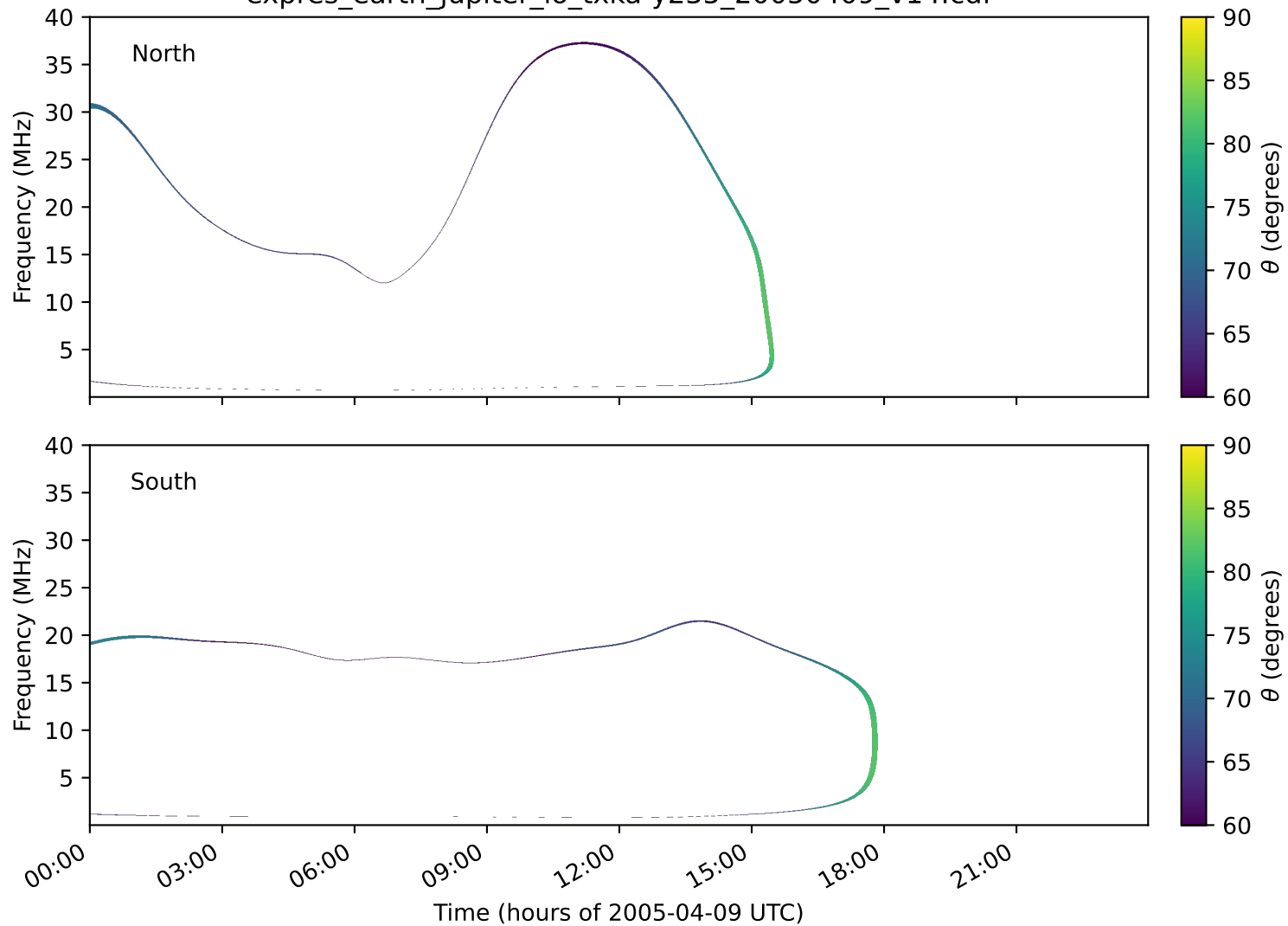
expres_earth_jupiter_io_txka-y235_20050409_v14.cdf
