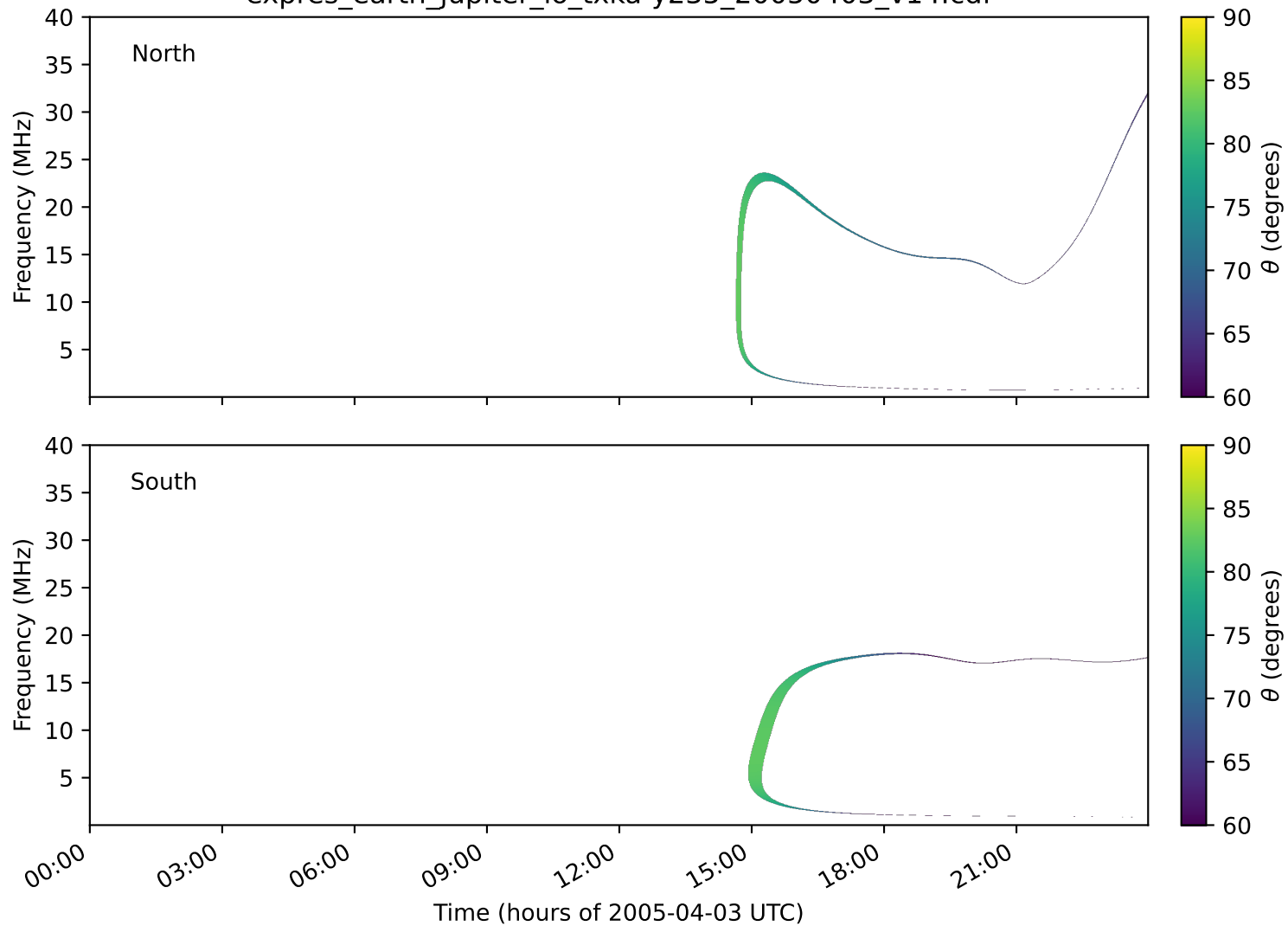
expres_earth_jupiter_io_txka-y235_20050403_v14.cdf
