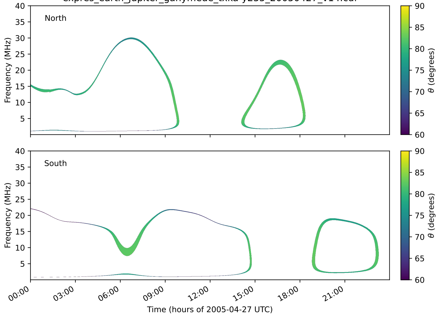
expres_earth_jupiter_ganymede_txka-y235_20050427_v14.cdf
