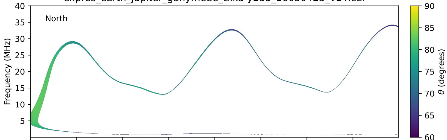
expres_earth_jupiter_ganymede_txka-y235_20050425_v14.cdf
