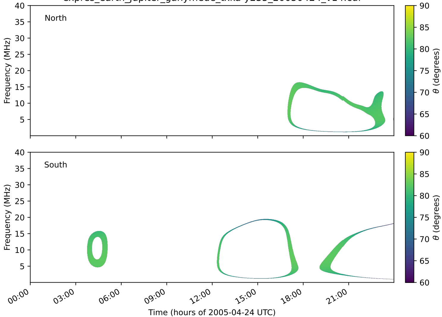
expres_earth_jupiter_ganymede_txka-y235_20050424_v14.cdf
