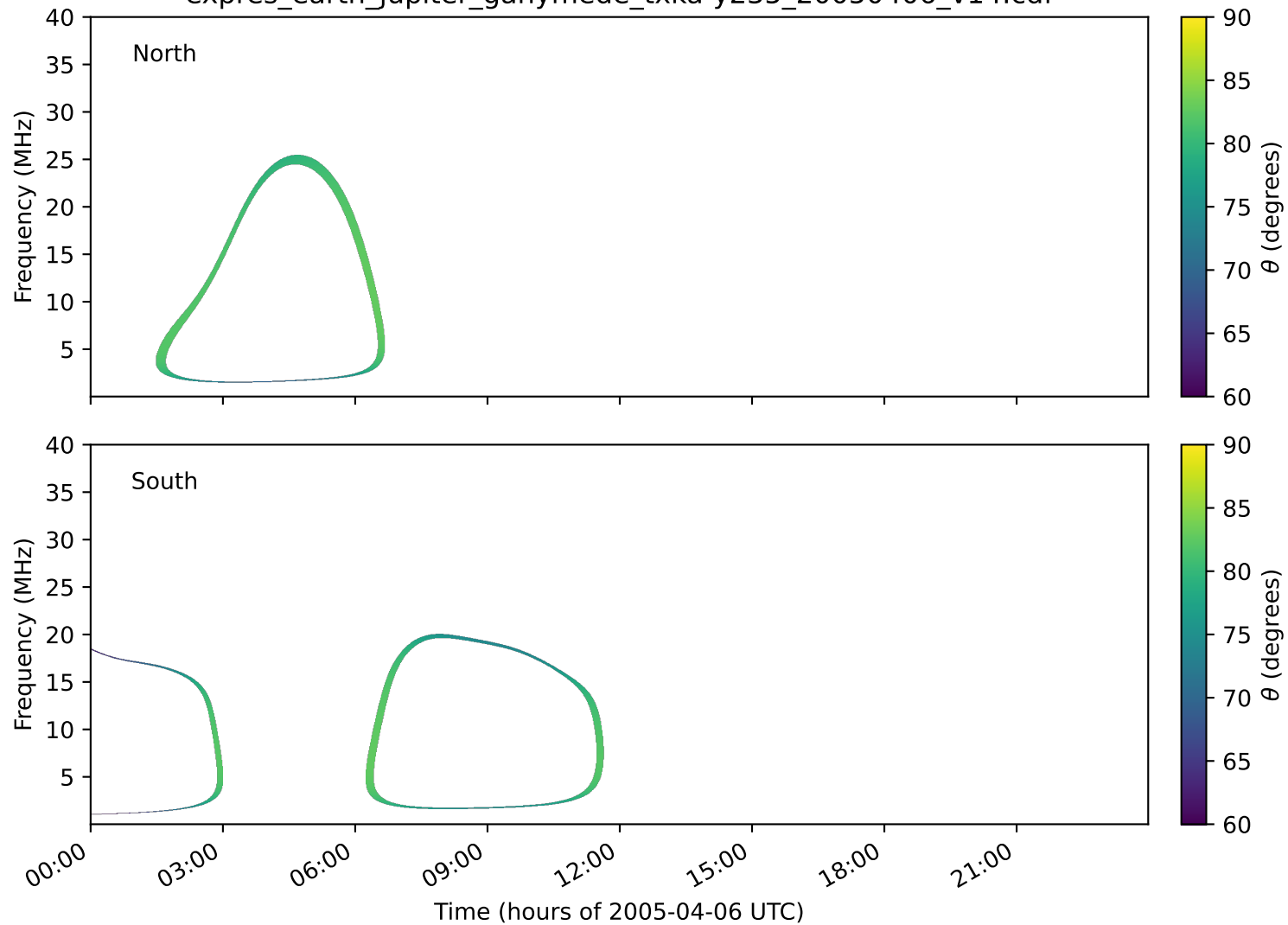
expres_earth_jupiter_ganymede_txka-y235_20050406_v14.cdf
