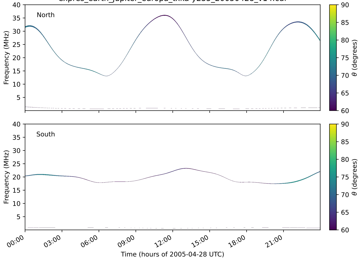
expres_earth_jupiter_europa_txka-y235_20050428_v14.cdf
