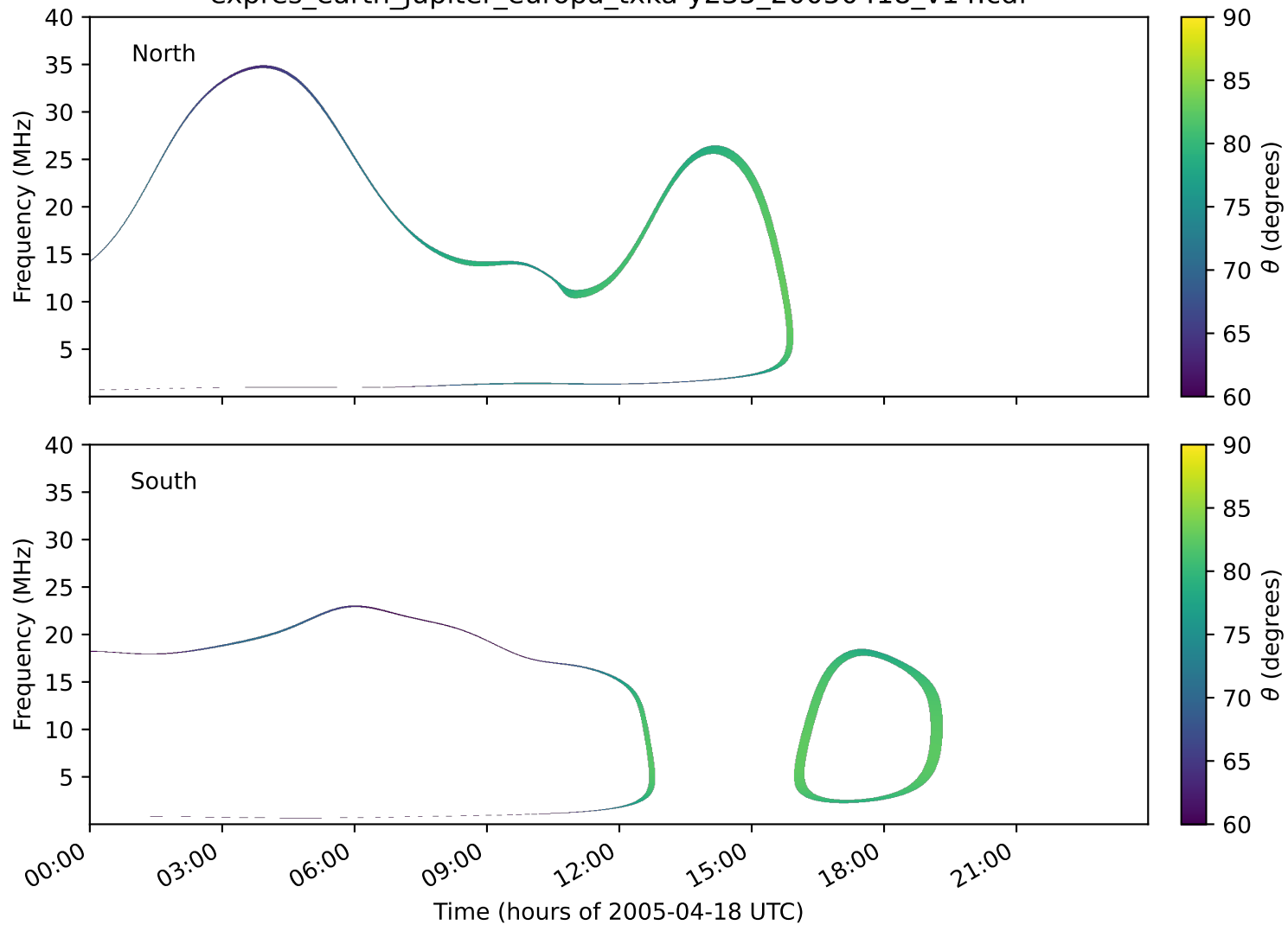
expres_earth_jupiter_europa_txka-y235_20050418_v14.cdf
