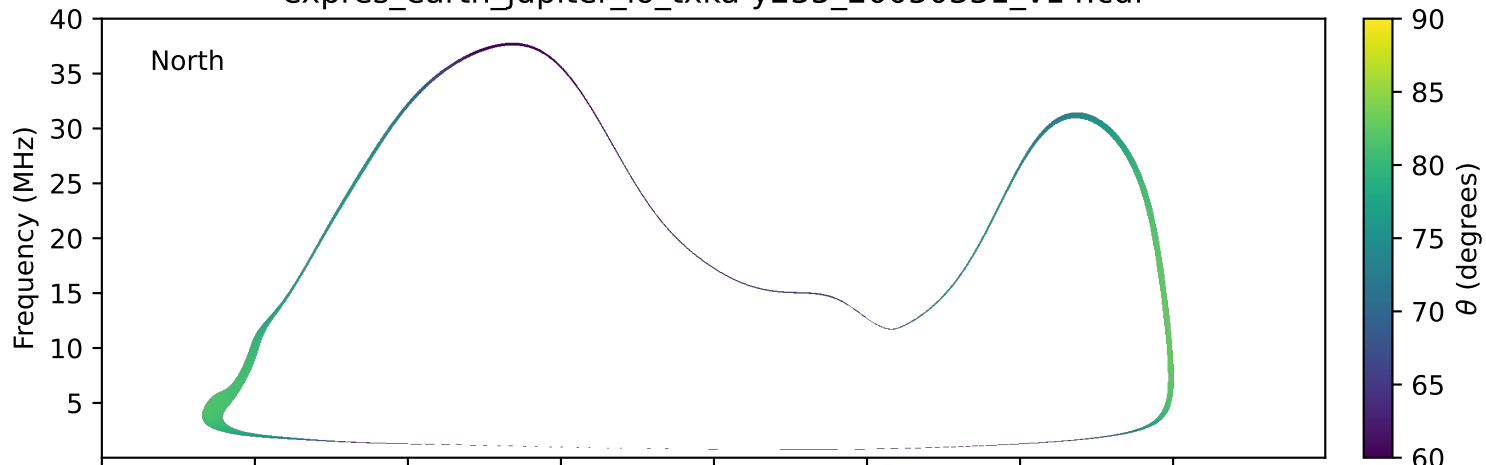
expres_earth_jupiter_io_txka-y235_20050331_v14.cdf
