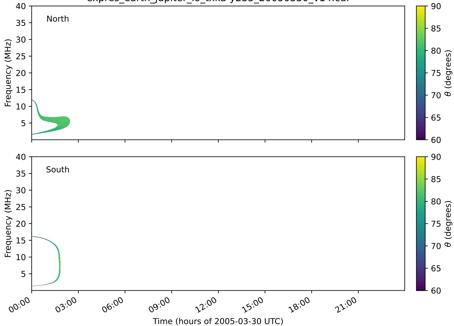
expres_earth_jupiter_io_txka-y235_20050330_v14.cdf
