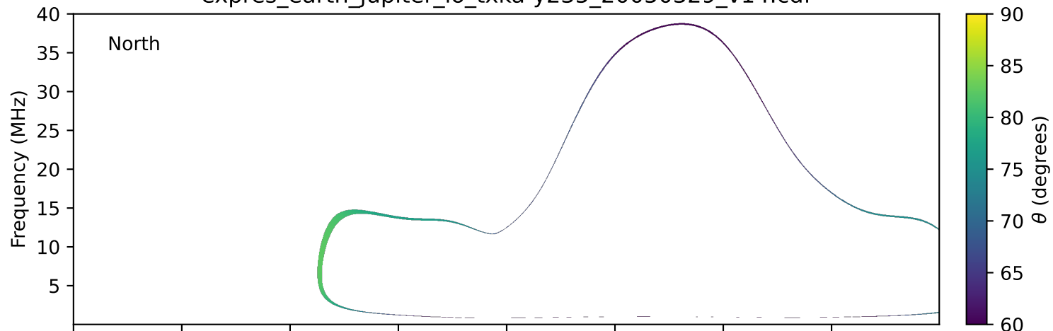
expres_earth_jupiter_io_txka-y235_20050329_v14.cdf
