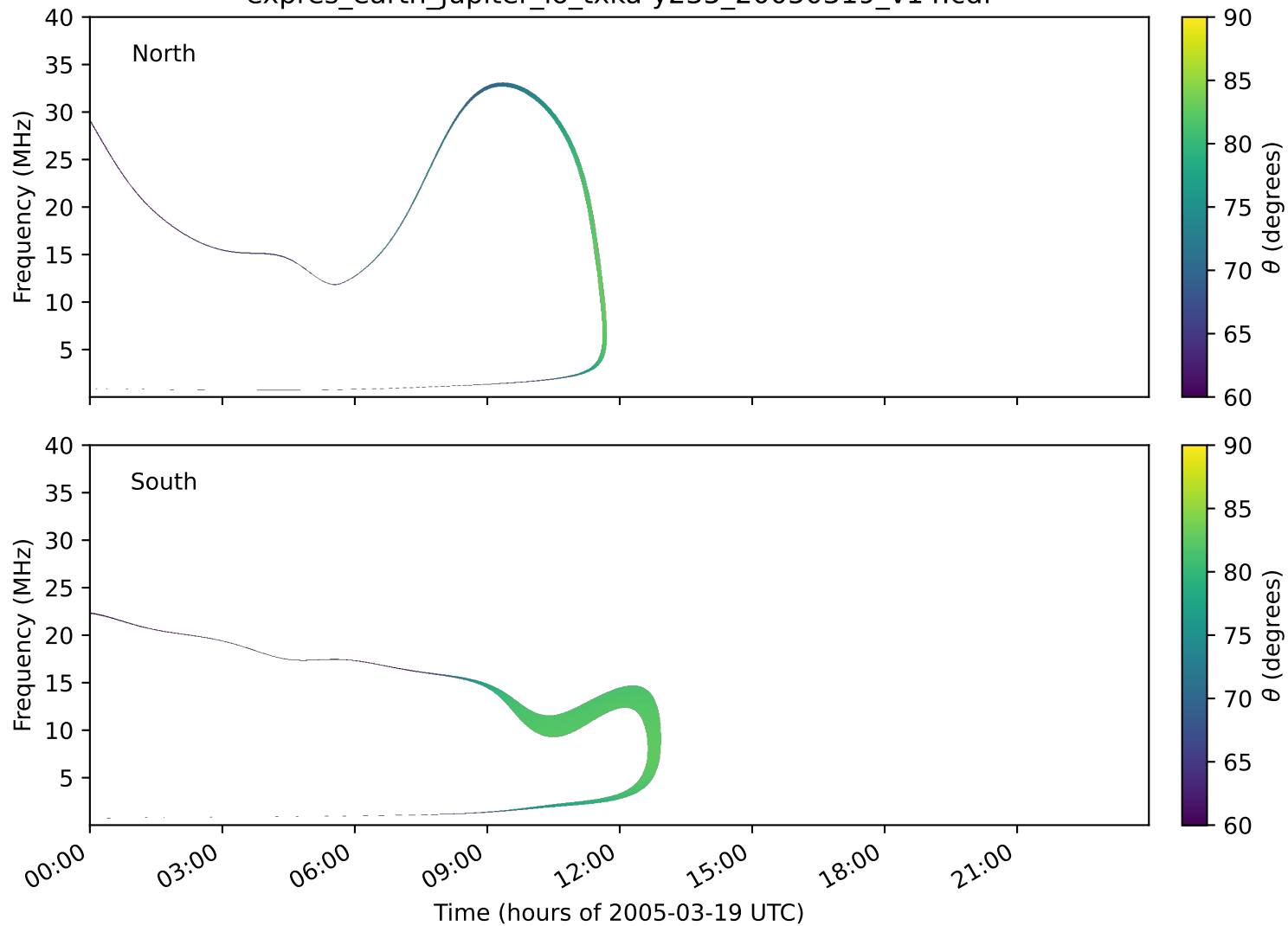
expres_earth_jupiter_io_txka-y235_20050319_v14.cdf
