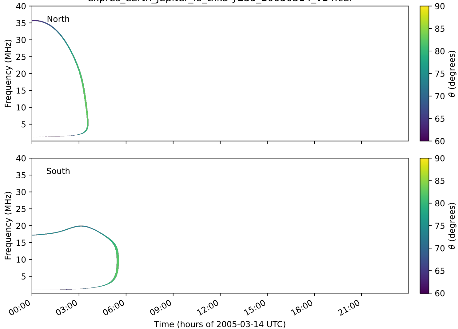
expres_earth_jupiter_io_txka-y235_20050314_v14.cdf
