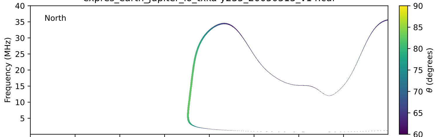
expres_earth_jupiter_io_txka-y235_20050313_v14.cdf
