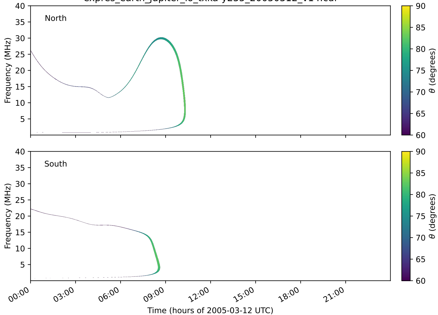
expres_earth_jupiter_io_txka-y235_20050312_v14.cdf
