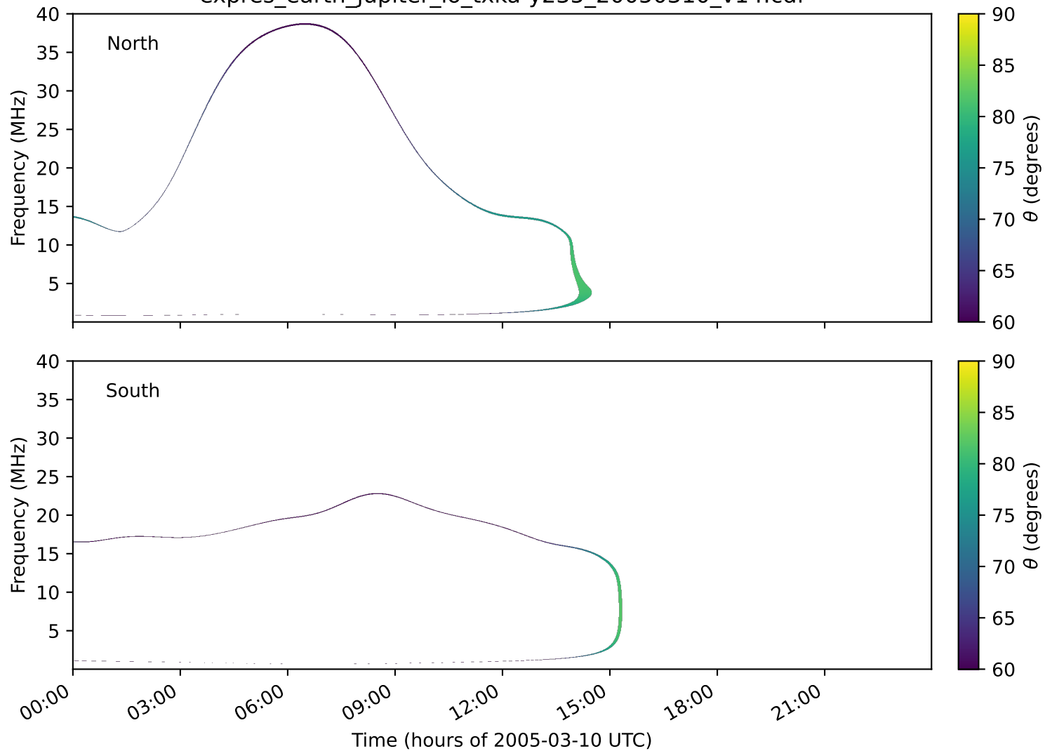
expres_earth_jupiter_io_txka-y235_20050310_v14.cdf
