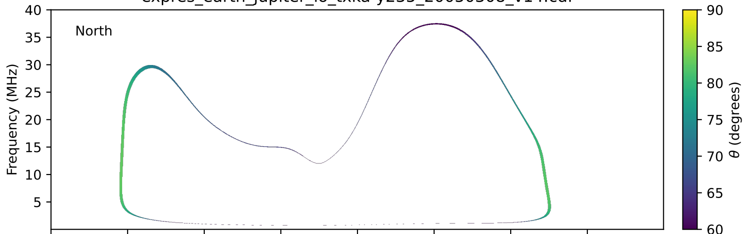
expres_earth_jupiter_io_txka-y235_20050308_v14.cdf
