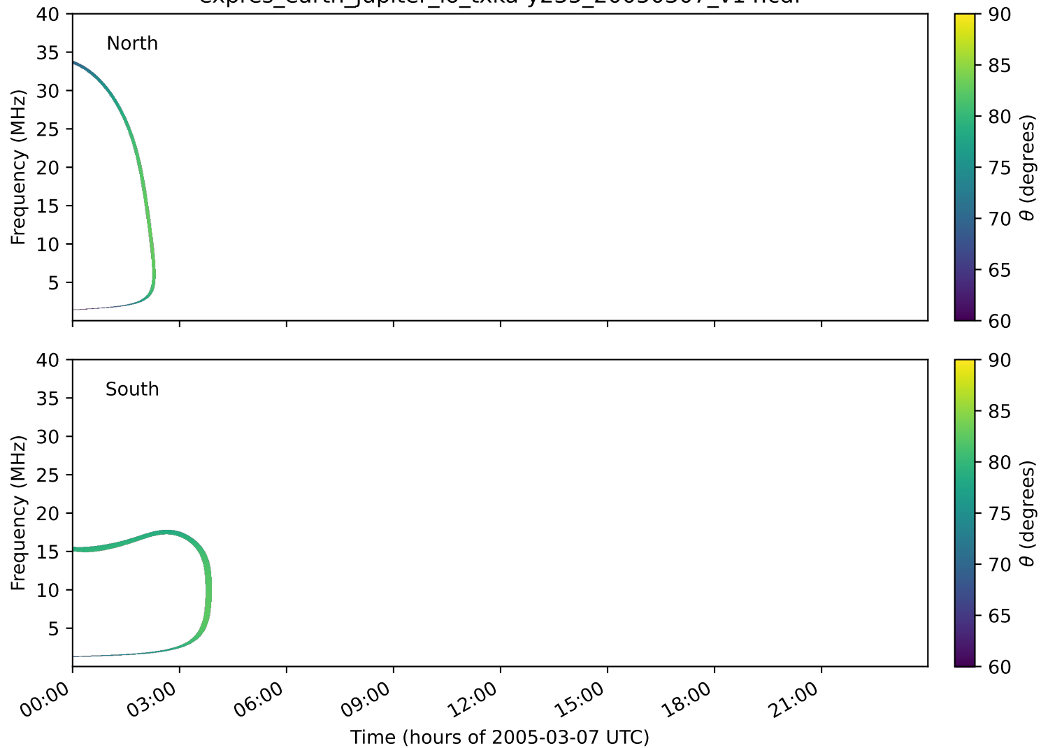
expres_earth_jupiter_io_txka-y235_20050307_v14.cdf
