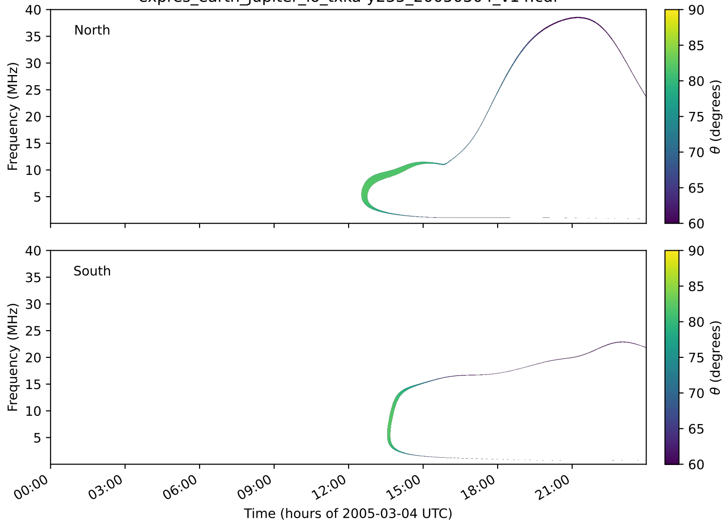
expres_earth_jupiter_io_txka-y235_20050304_v14.cdf
