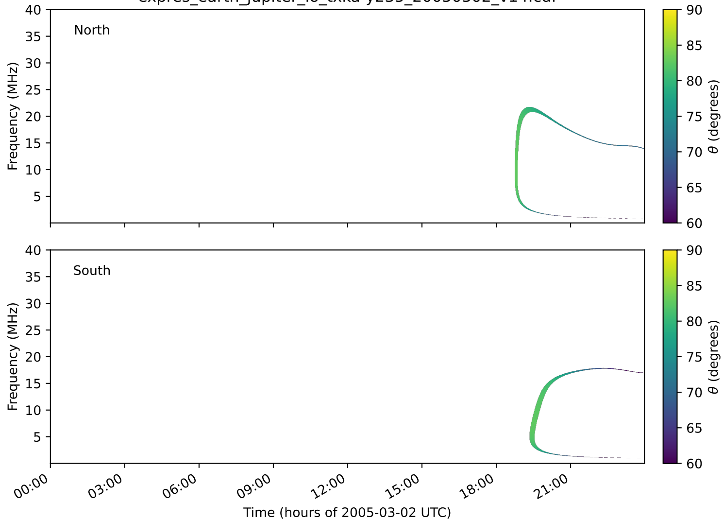
expres_earth_jupiter_io_txka-y235_20050302_v14.cdf
