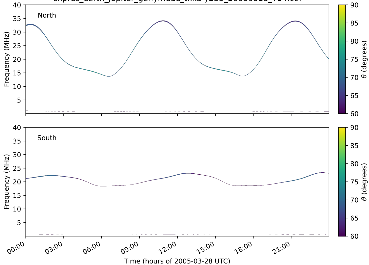
expres_earth_jupiter_ganymede_txka-y235_20050328_v14.cdf
