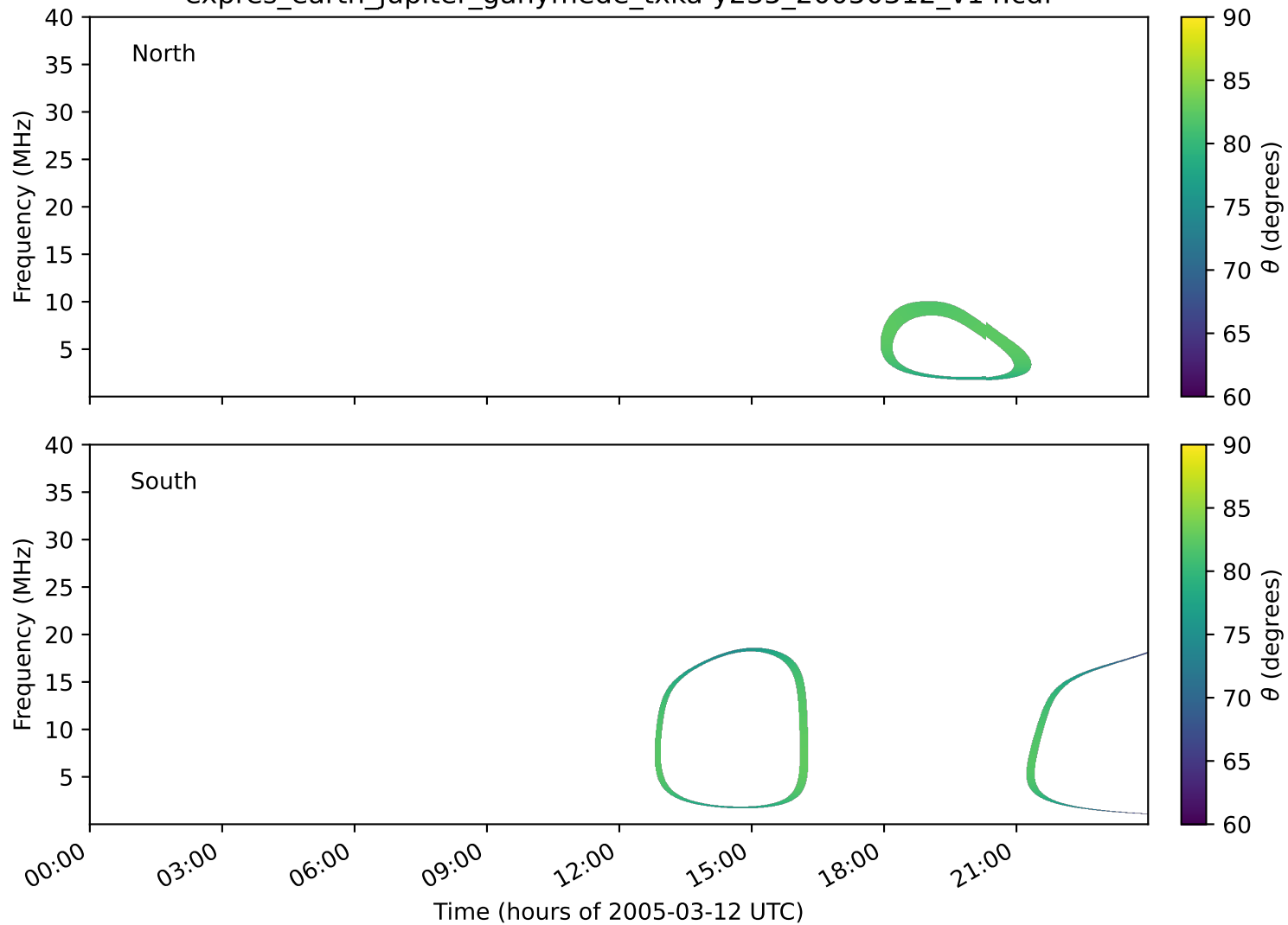
expres_earth_jupiter_ganymede_txka-y235_20050312_v14.cdf
