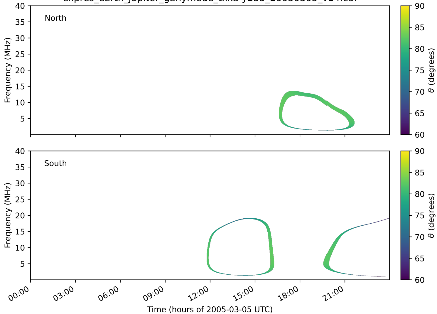
expres_earth_jupiter_ganymede_txka-y235_20050305_v14.cdf
