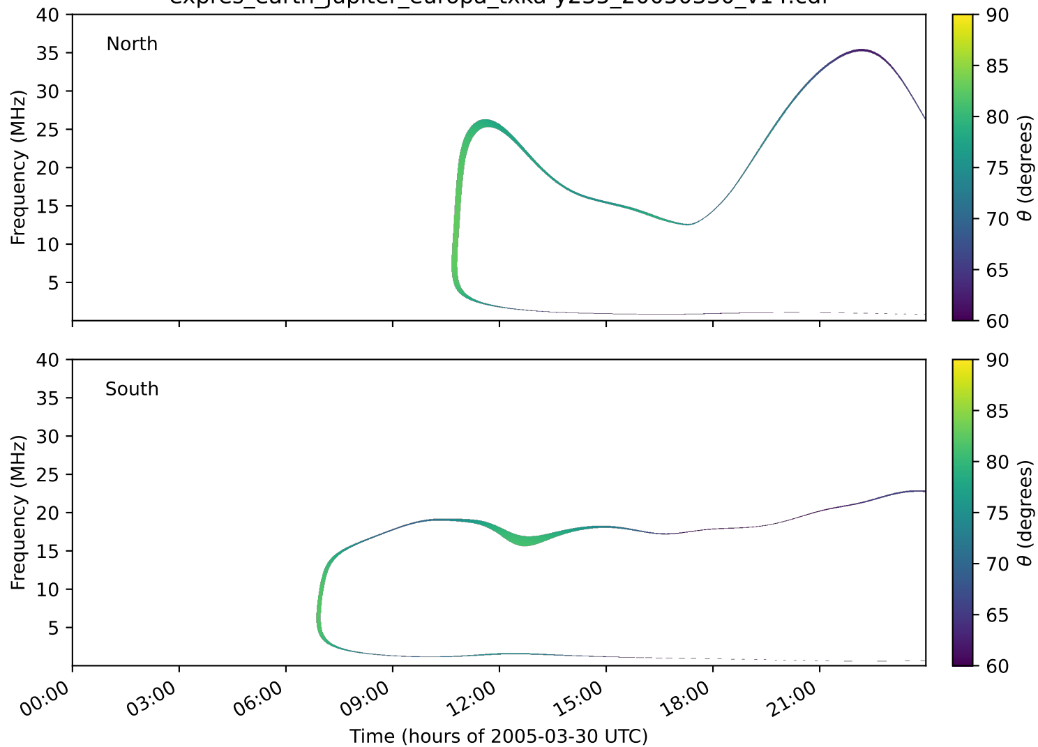
expres_earth_jupiter_europa_txka-y235_20050330_v14.cdf
