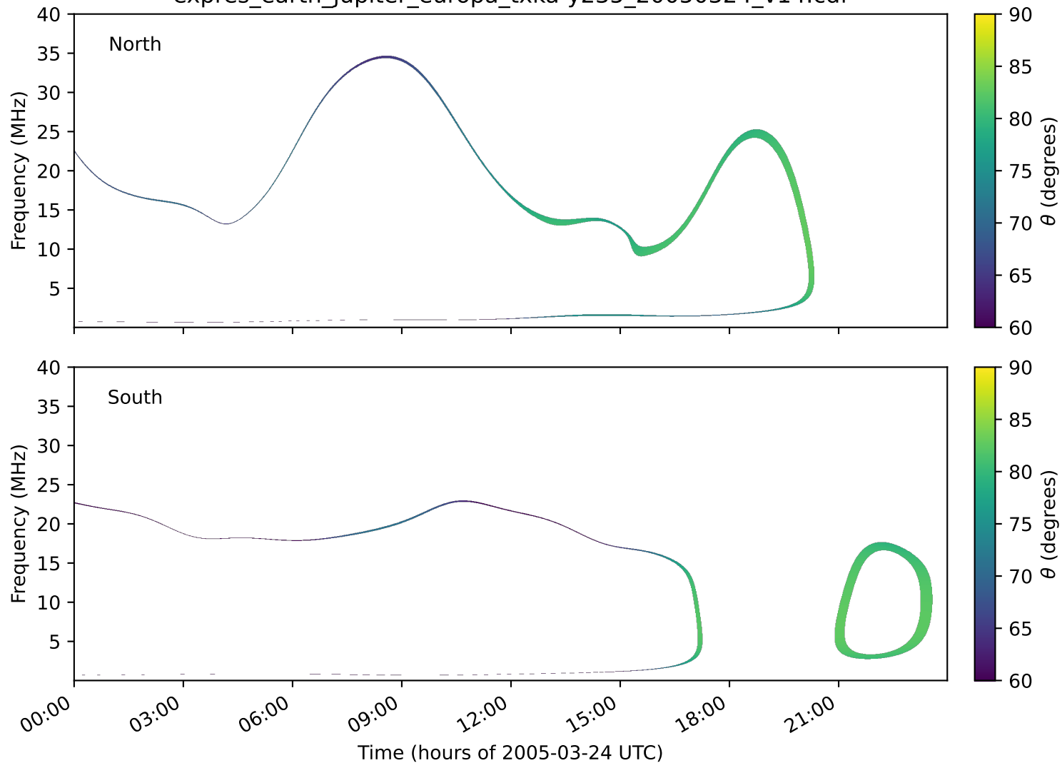
expres_earth_jupiter_europa_txka-y235_20050324_v14.cdf
