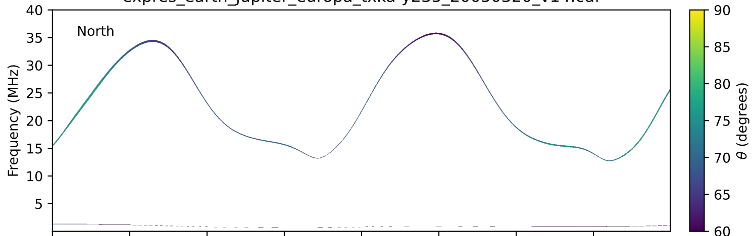
expres_earth_jupiter_europa_txka-y235_20050320_v14.cdf
