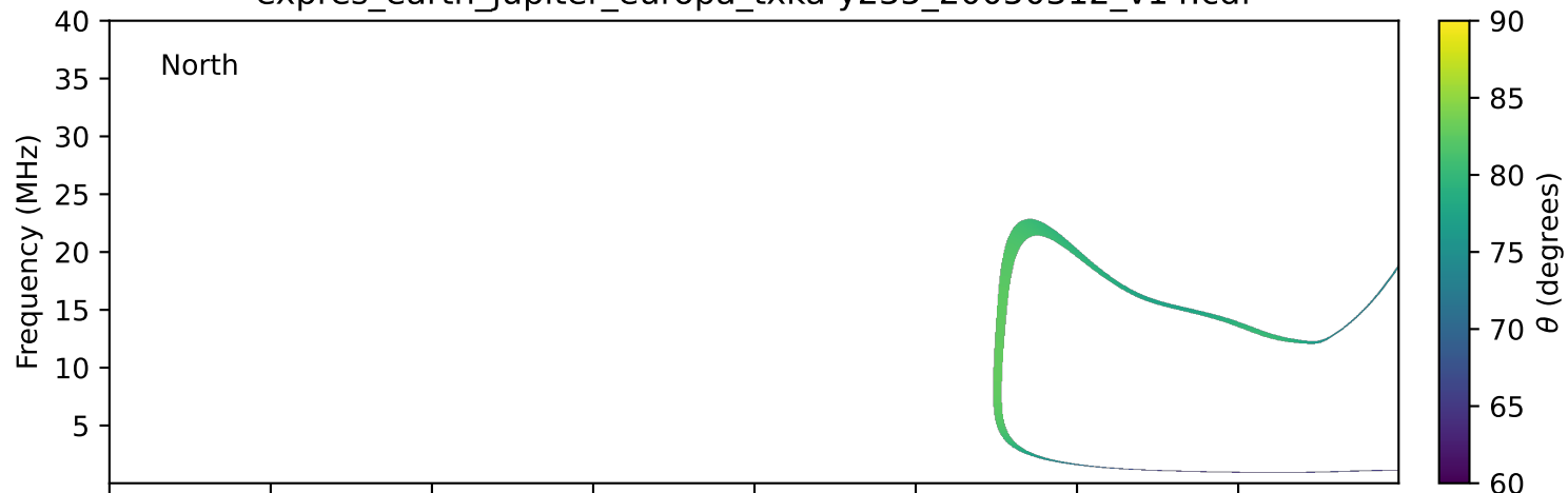
expres_earth_jupiter_europa_txka-y235_20050312_v14.cdf
