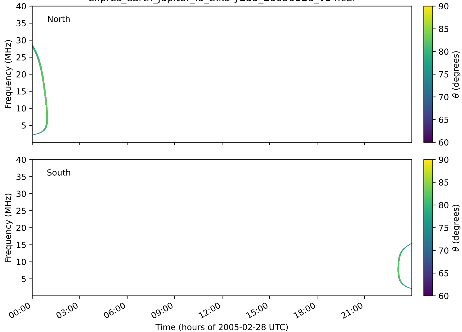
expres_earth_jupiter_io_txka-y235_20050228_v14.cdf
