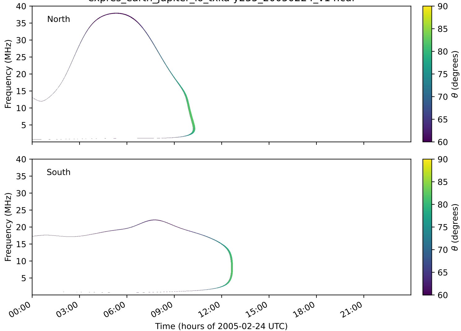
expres_earth_jupiter_io_txka-y235_20050224_v14.cdf
