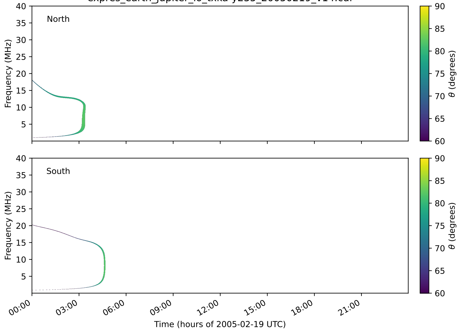
expres_earth_jupiter_io_txka-y235_20050219_v14.cdf
