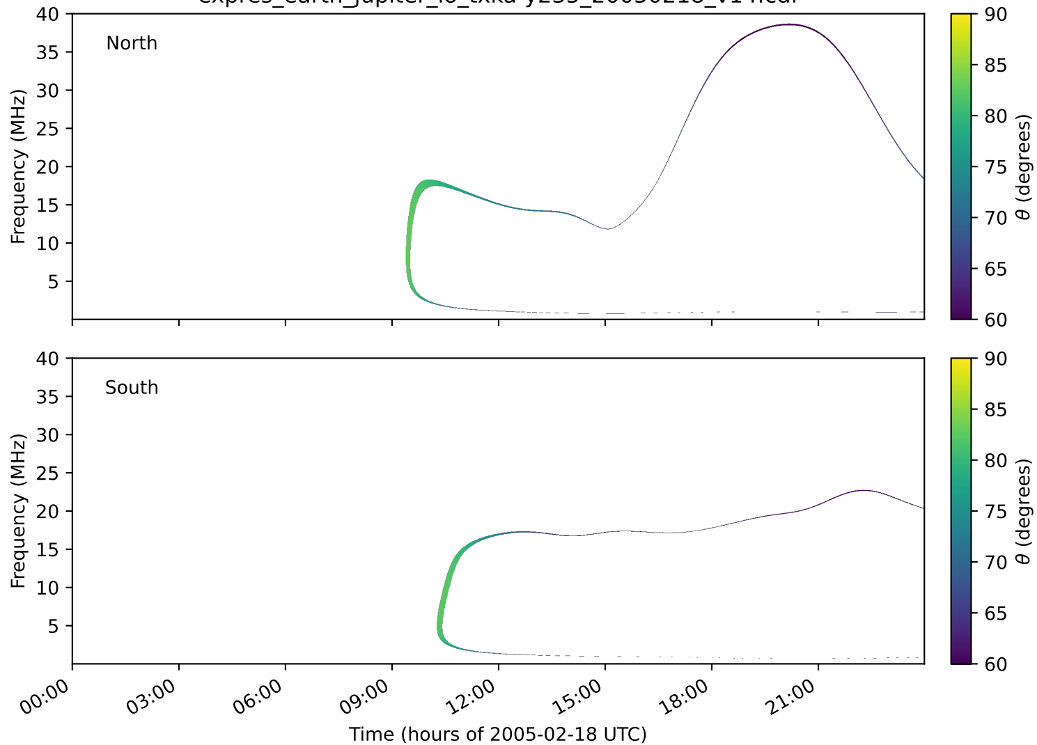
expres_earth_jupiter_io_txka-y235_20050218_v14.cdf
