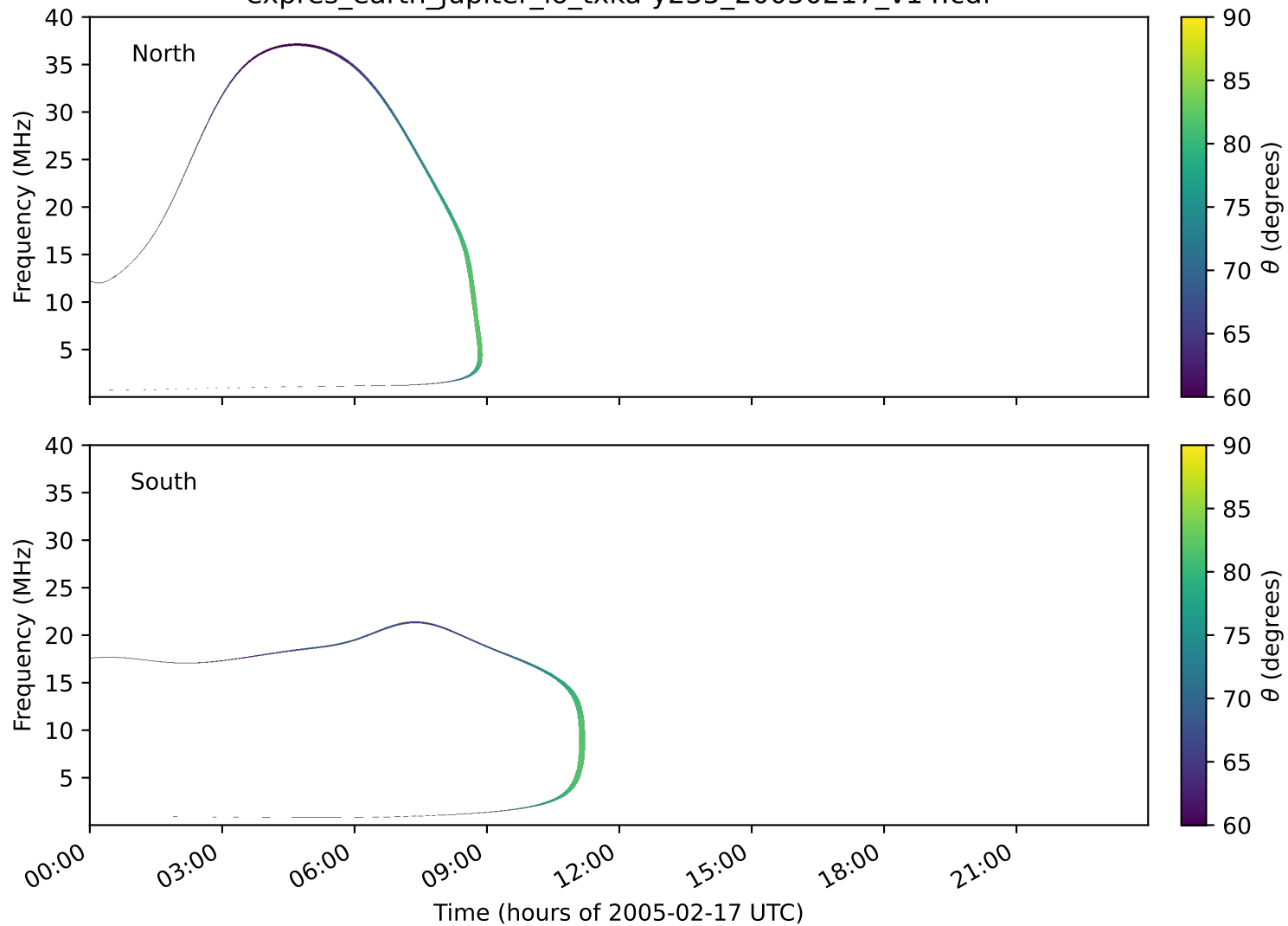
expres_earth_jupiter_io_txka-y235_20050217_v14.cdf
