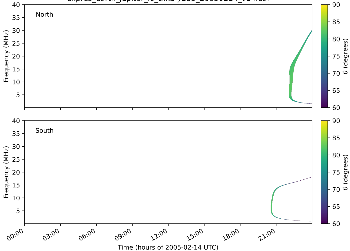
expres_earth_jupiter_io_txka-y235_20050214_v14.cdf
