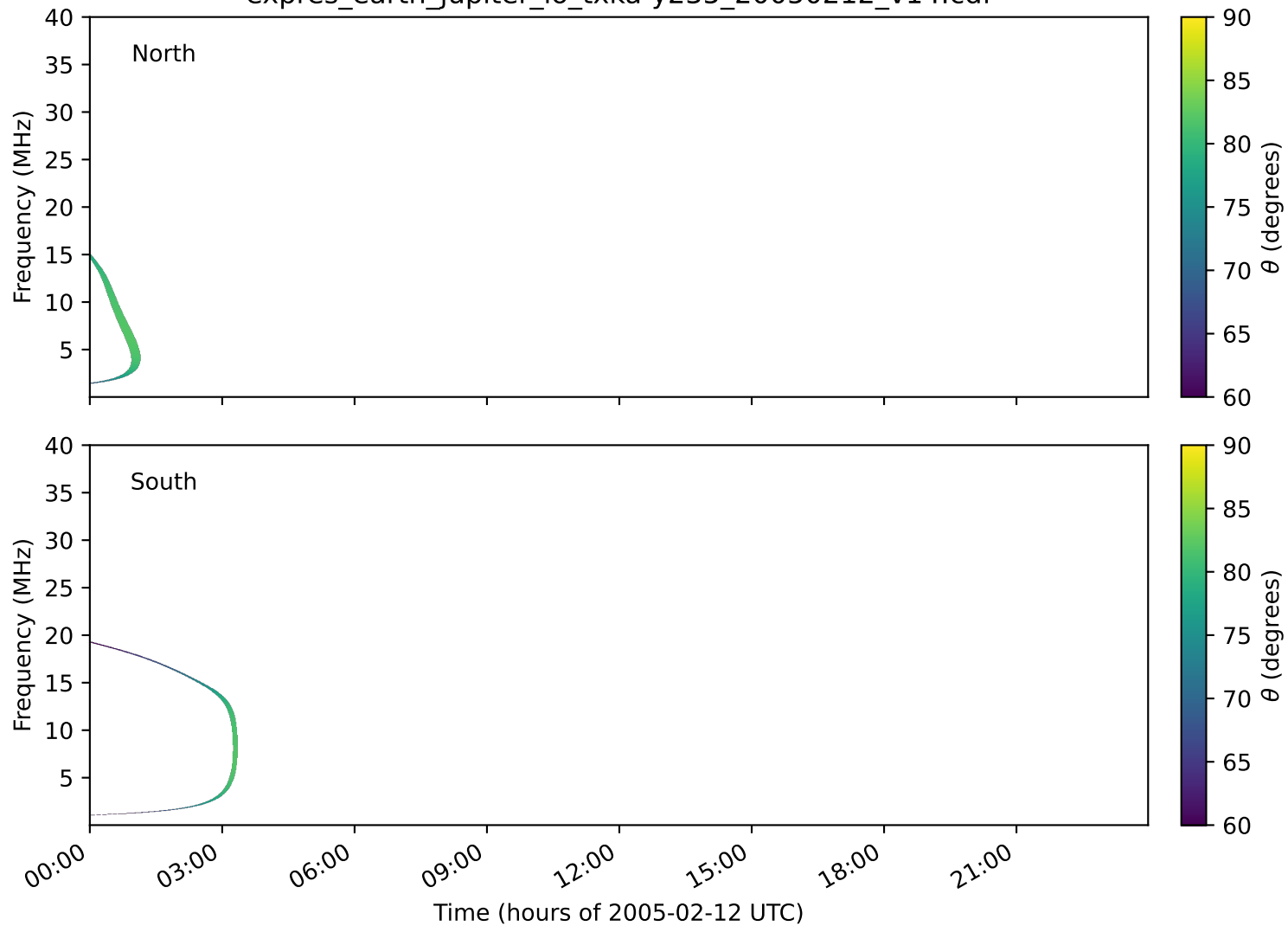
expres_earth_jupiter_io_txka-y235_20050212_v14.cdf
