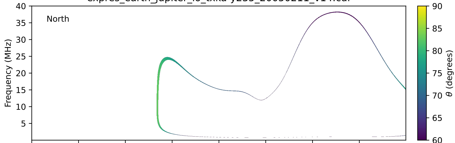
expres_earth_jupiter_io_txka-y235_20050211_v14.cdf
