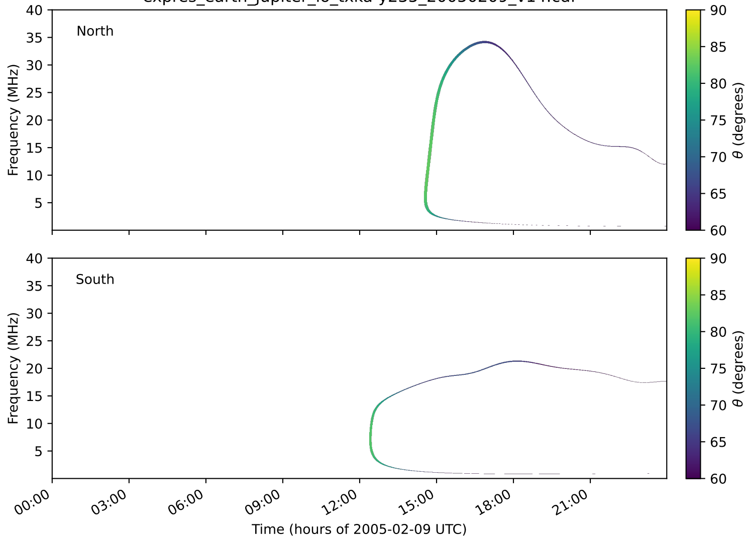
expres_earth_jupiter_io_txka-y235_20050209_v14.cdf
