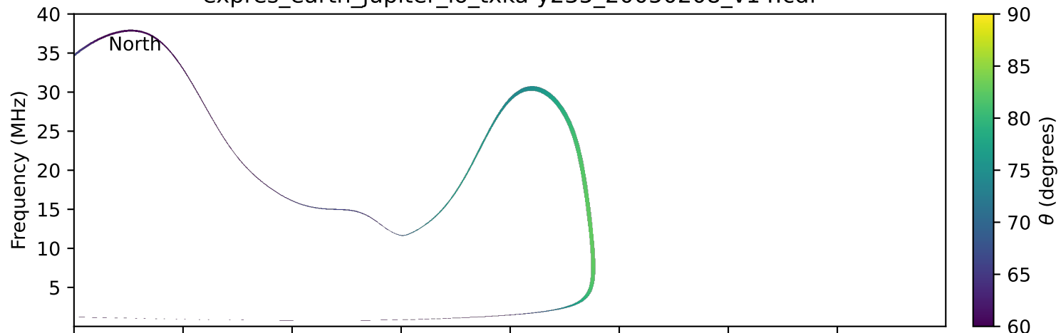
expres_earth_jupiter_io_txka-y235_20050208_v14.cdf
