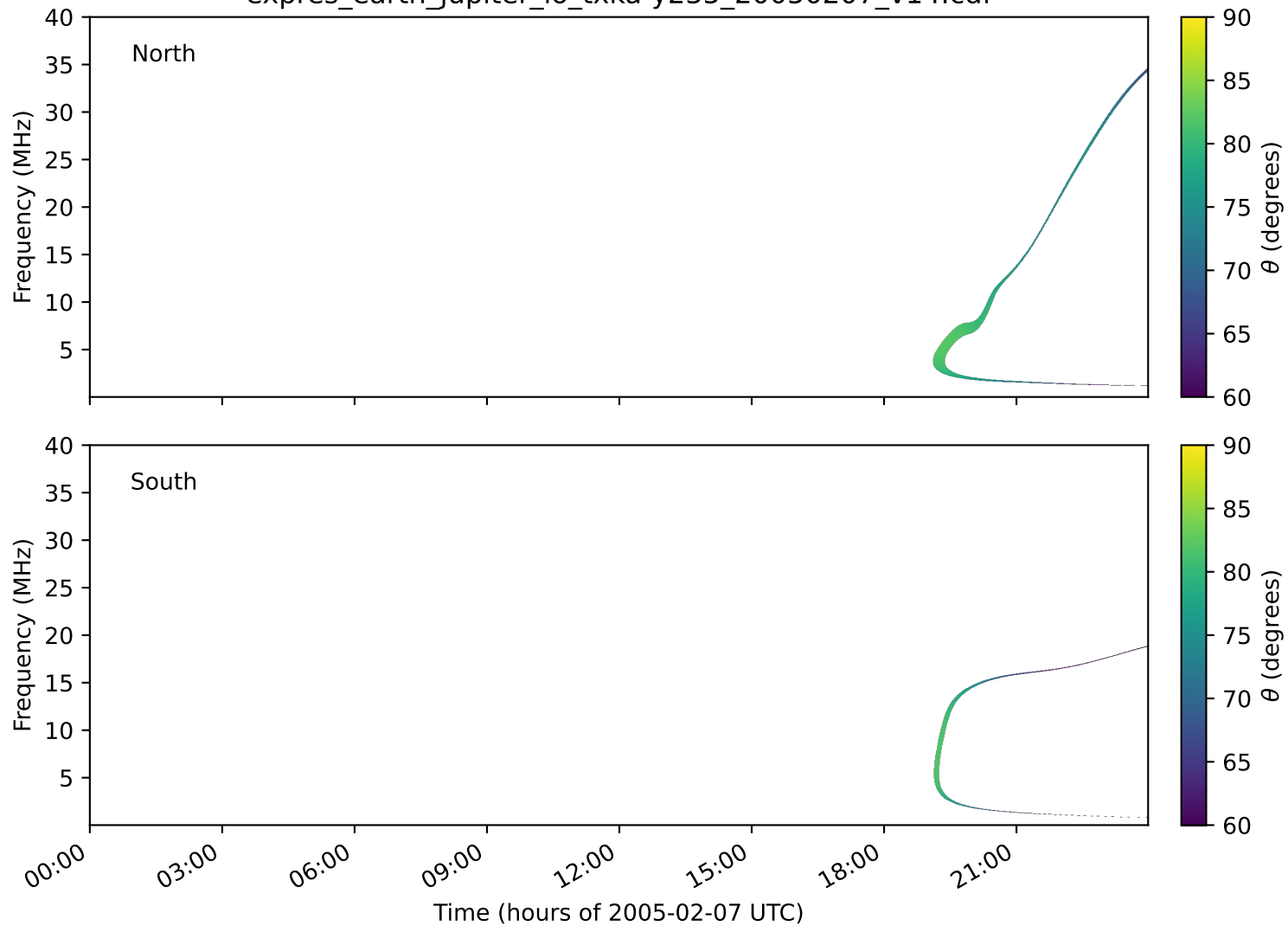
expres_earth_jupiter_io_txka-y235_20050207_v14.cdf
