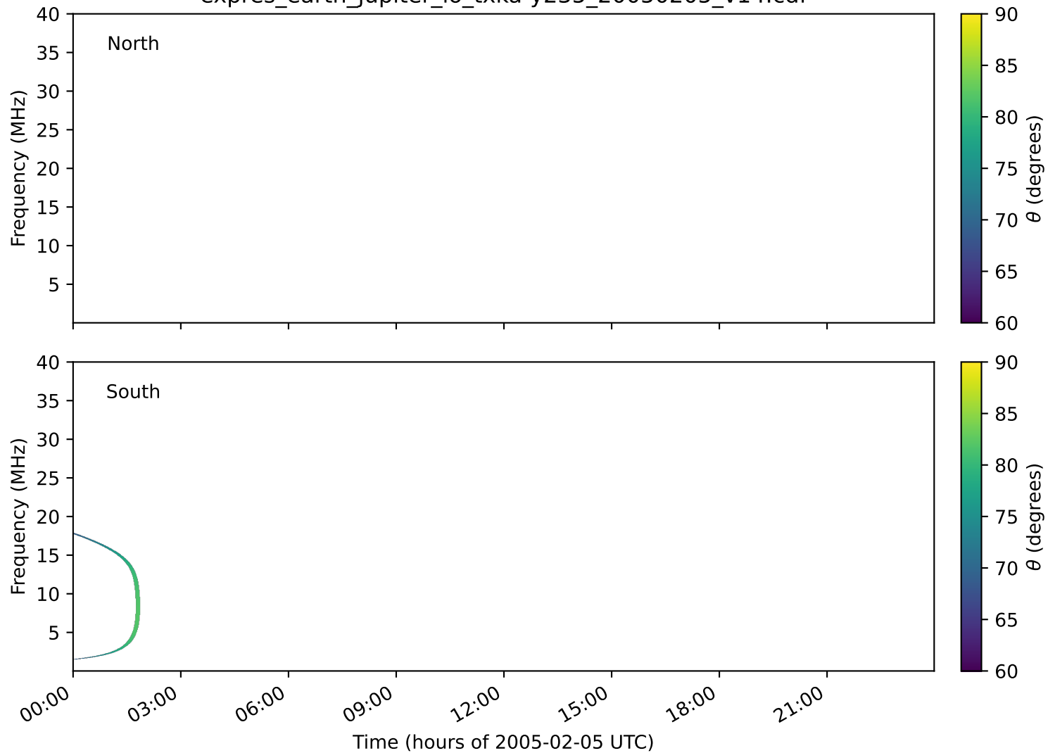
expres_earth_jupiter_io_txka-y235_20050205_v14.cdf
