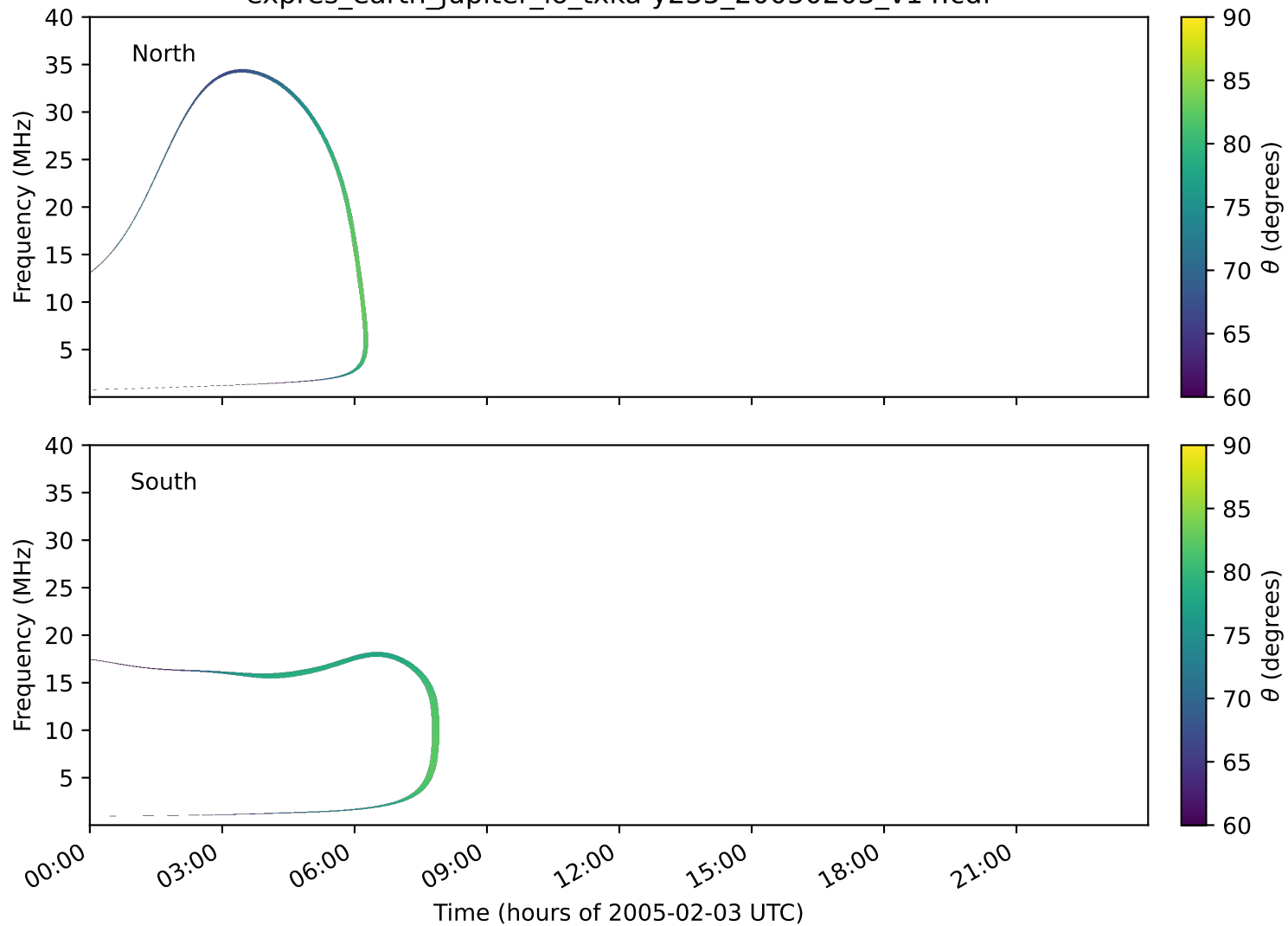
expres_earth_jupiter_io_txka-y235_20050203_v14.cdf
